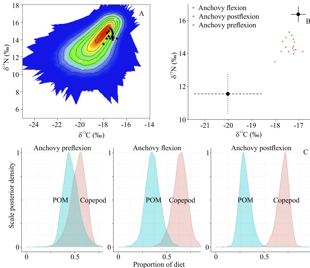
Figure 5. A) Monte Carlo simulation of the mixing region for a model with two stable isotopes and potential sources (calanoid copepods < 1 mm and particulate organic matter –POM) created using the procedure described by Smith et al. (2013). A) Trophic enrichment factors and errors were \delta^{15}\text{N} : 3.0 \pm 0.3 SD; \delta^{13}\text{C} : 1.0 \pm 0.3 SD. B) Biplot of corrected \delta^{15}\text{N} and \delta^{13}\text{C} values for consumers ( Engraulis anchoita larvae by developmental stages) and potential prey (calanoid copepods < 1 mm and POM) created with MixSIAR. Error bars represent 95% confidence intervals and incorporate error in prey isotopic signal and trophic enrichment factors ( \delta^{15}\text{N} : 3.4 \pm 0.3 SD; \delta^{13}\text{C} : 1.0 \pm 0.3 SD). C) Posterior distributions of the probability of prey item contribution (calanoid copepods < 1 mm and POM) for each developmental stage of Engraulis anchoita (preflexion, flexion, and postflexion) in the autumn season.
